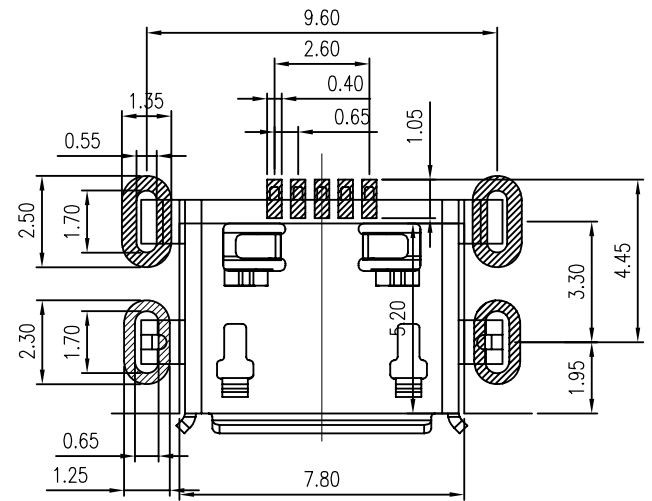
RECOMMENDED PCB LAYOUT(TOP VIEW) GENERAL TOLERANCES:±0.05
